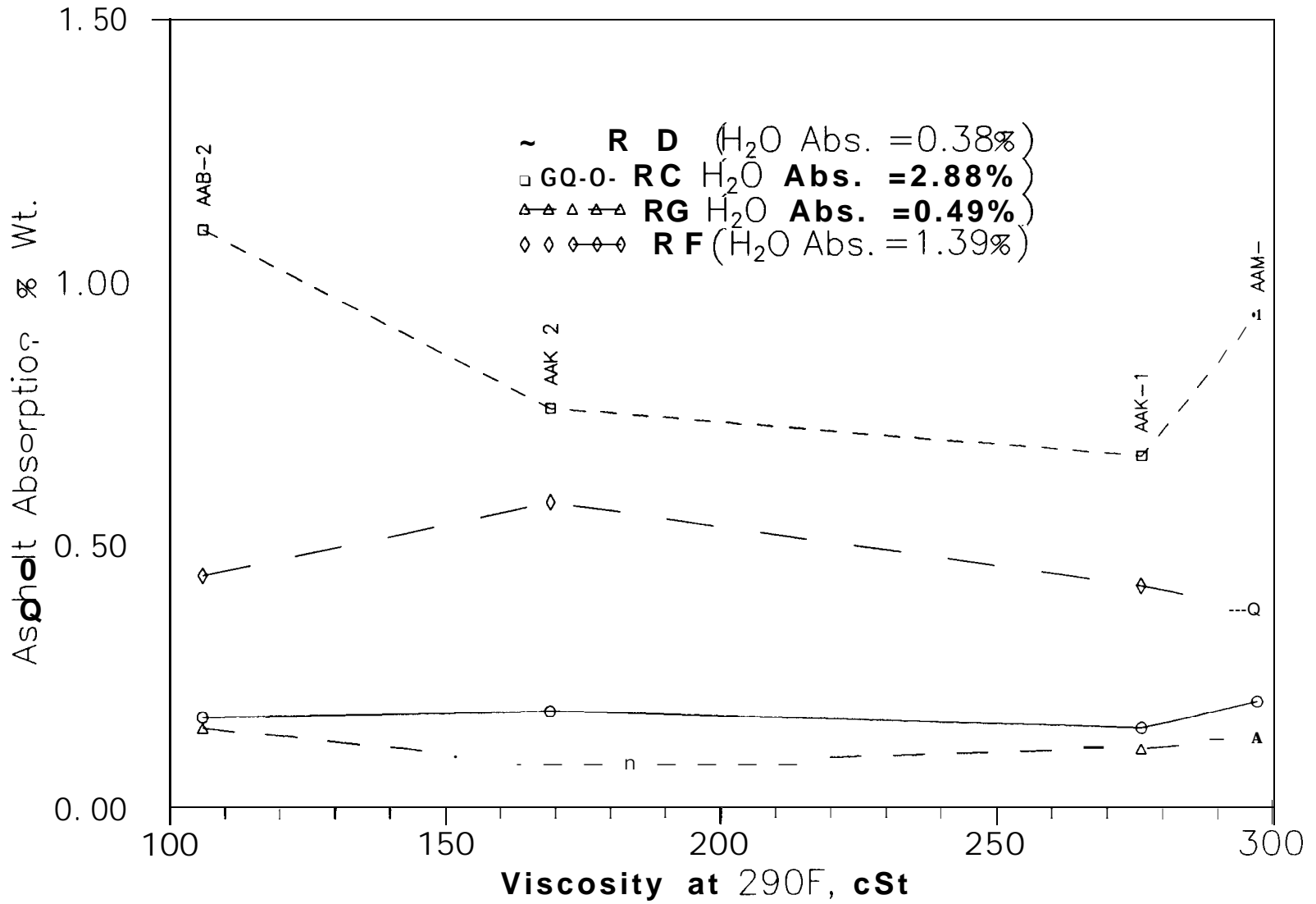
Fig. 1 - Asphalt Absorption vs. Viscosity of Asphalt Cement
